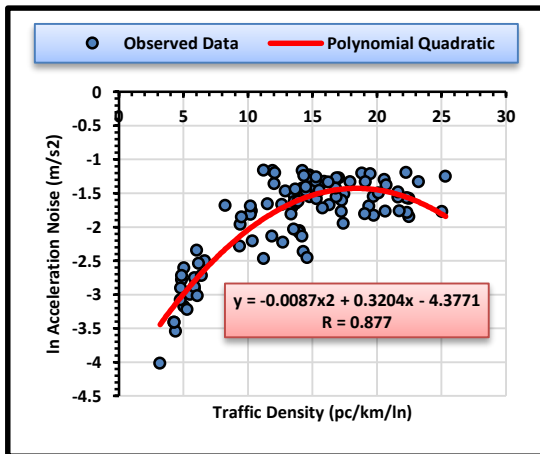
Fig. 5: Effect of Traffic Density on the Transformed Acceleration Noise on Multi-Lanes Arterial Roads
