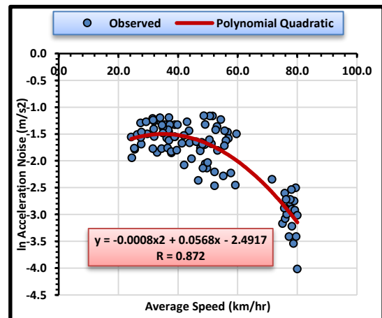
Fig. 4: Effect of Average Speed on the Transformed Acceleration Noise on Multi-Lanes Arterial Roads
