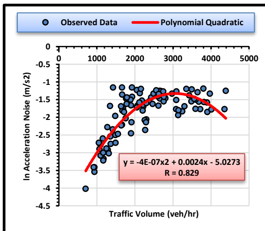
Fig. 3: Effect of Traffic Volume on the Transformed Acceleration Noise on Multi-Lanes Arterial Roads
